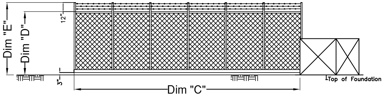
BARRIER STYLE "A" STYLE 1810
