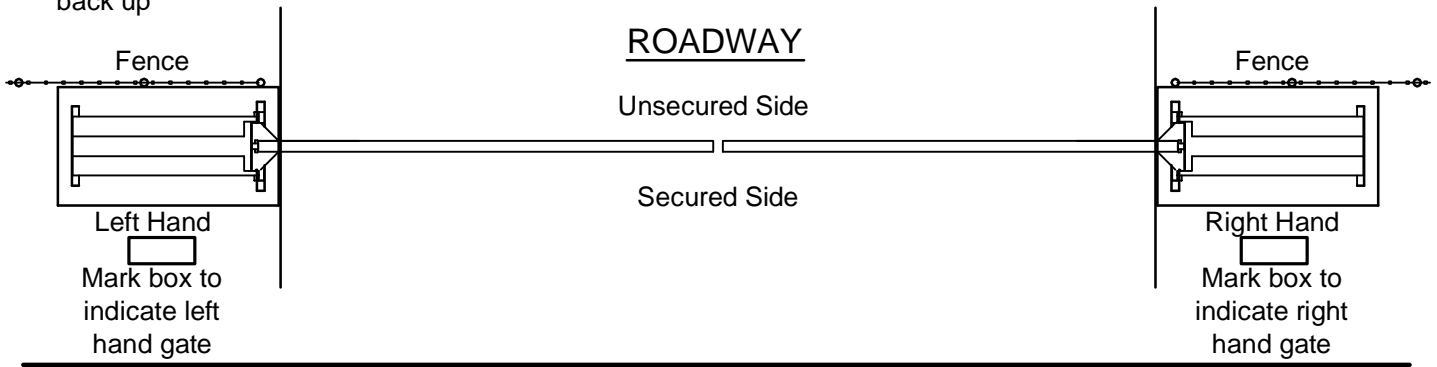
BARRIER STYLE "A" STYLE 1810
